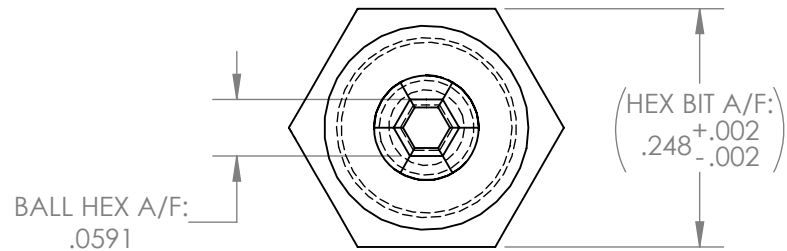
DETAIL A SCALE 5 : 1
